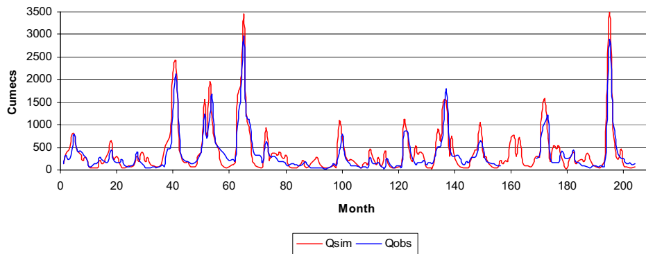
Fig. 10. Tejo: simulation results at Almourol station for the period 1973–90
