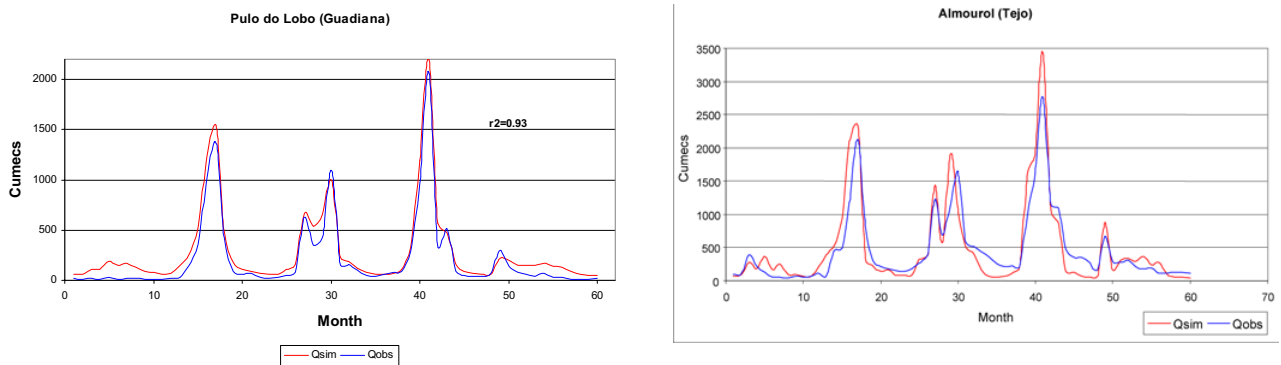
Fig. 9. Validation results for Guadiana and Tejo basins
