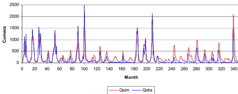
Fig. 11. Guadiana: simulation results at Pulo Do Lobo station for the period 1961–90
