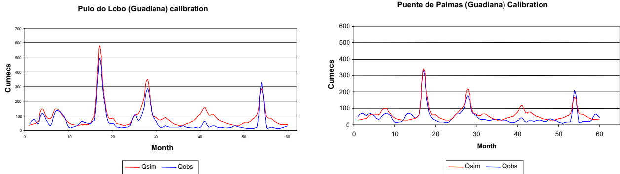
Fig. 7. Hydrographs for model calibration for the Guadiana catchment
