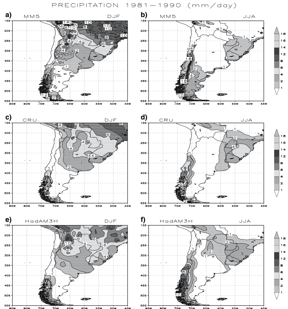
Fig. 4 Average precipitation for the period 1981–1990 from the regional model (a, b), observations (c, d) and the global model (e, f) for summer (DJF) and winter (JJA), respectively. Minimum contour is 1 mm/day. Contours are drawn every 2 mm/day for values greater than 2 mm/day
